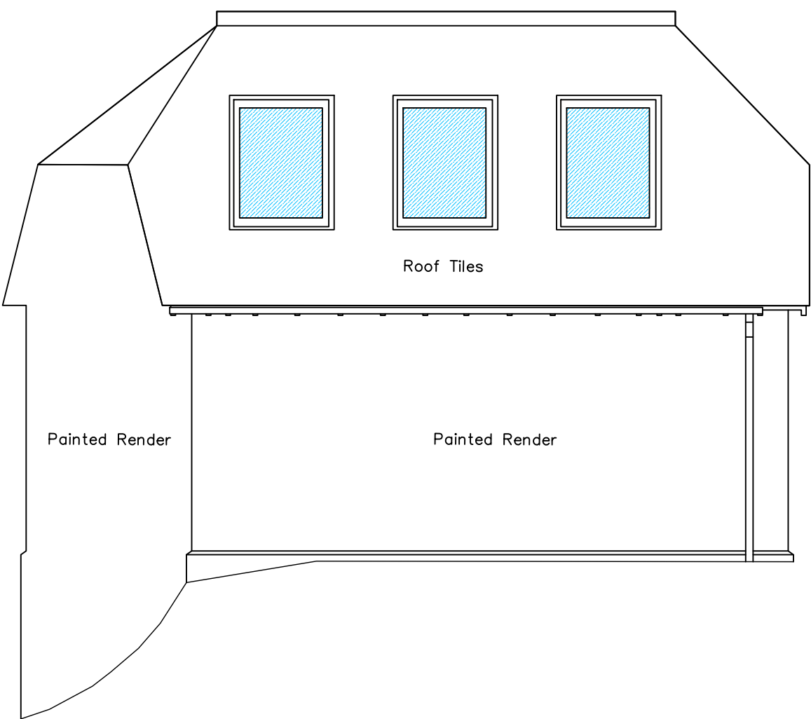
Existing North Elevation Datum 67.00m
