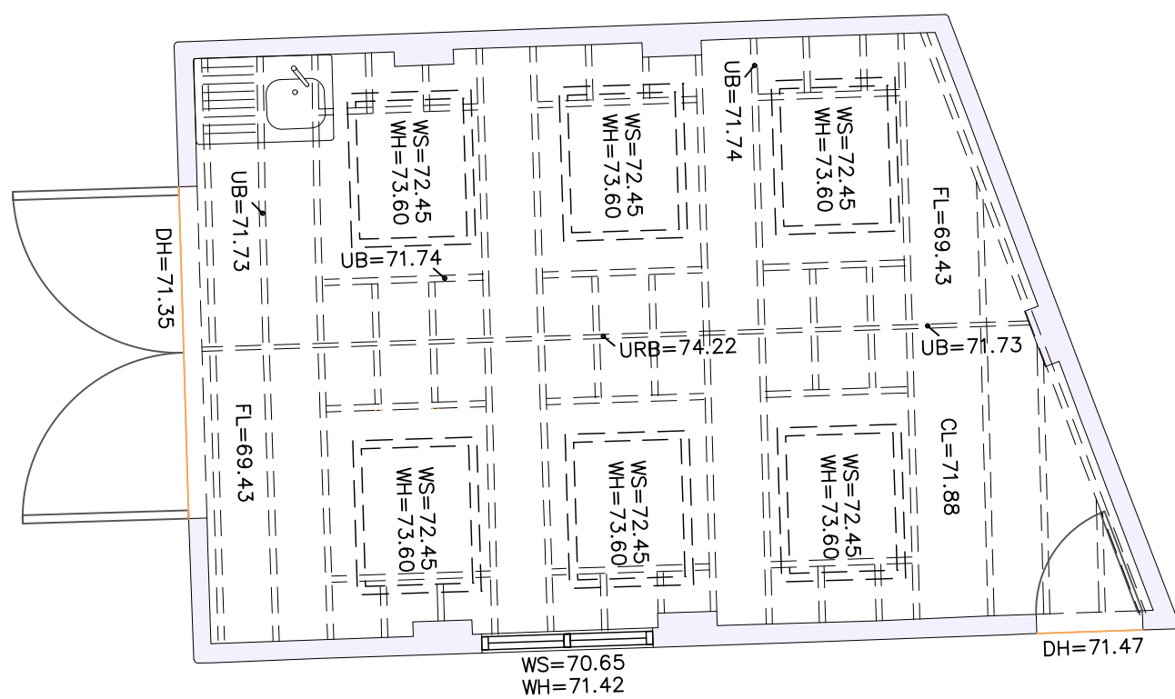
Existing Garage Plan
