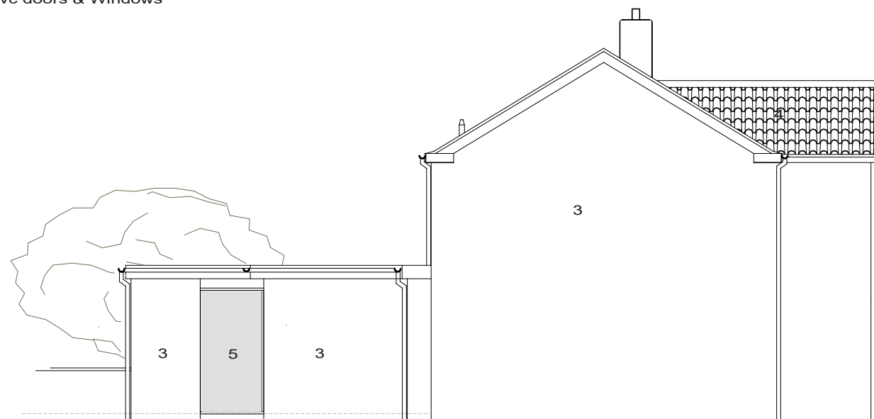
3- WEST PROPOSED ELEVATION
