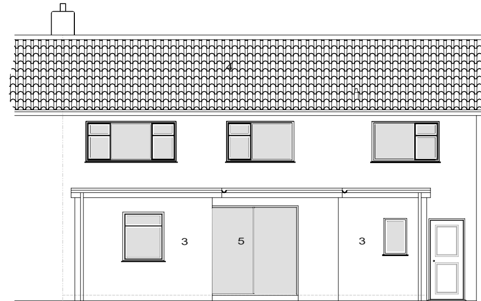
2- NORTH PROPOSED ELEVATION (FACING REAR GARDEN)
