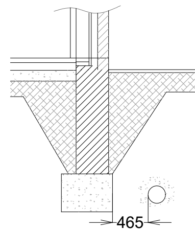
SECTION E-E
