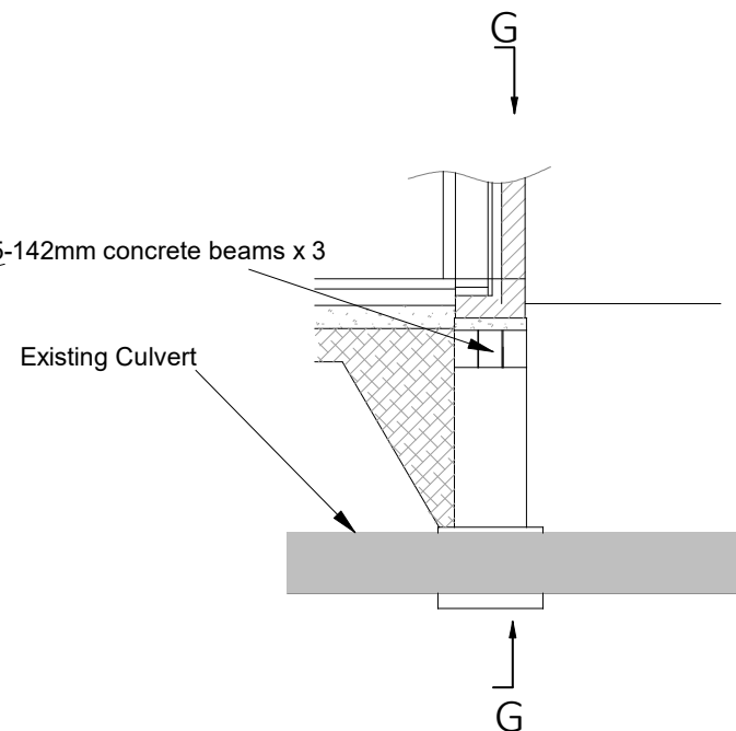
SECTION G-G
