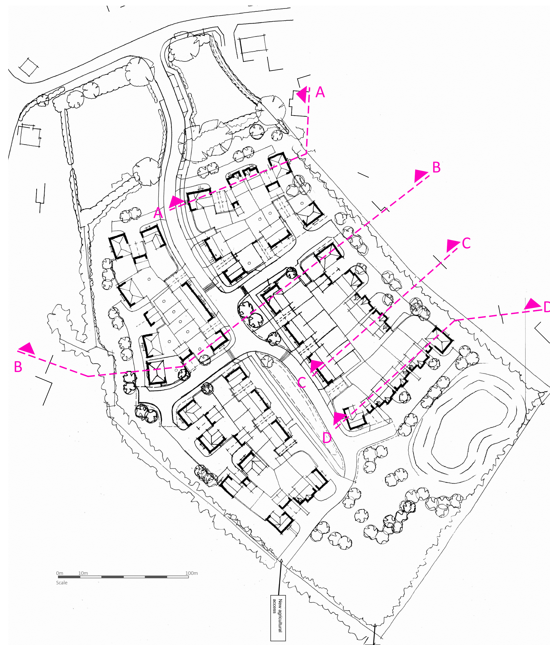
Proposed layout showing the location of site sections Not to recognised scale
