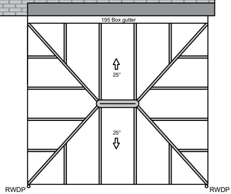
Roof Layout
