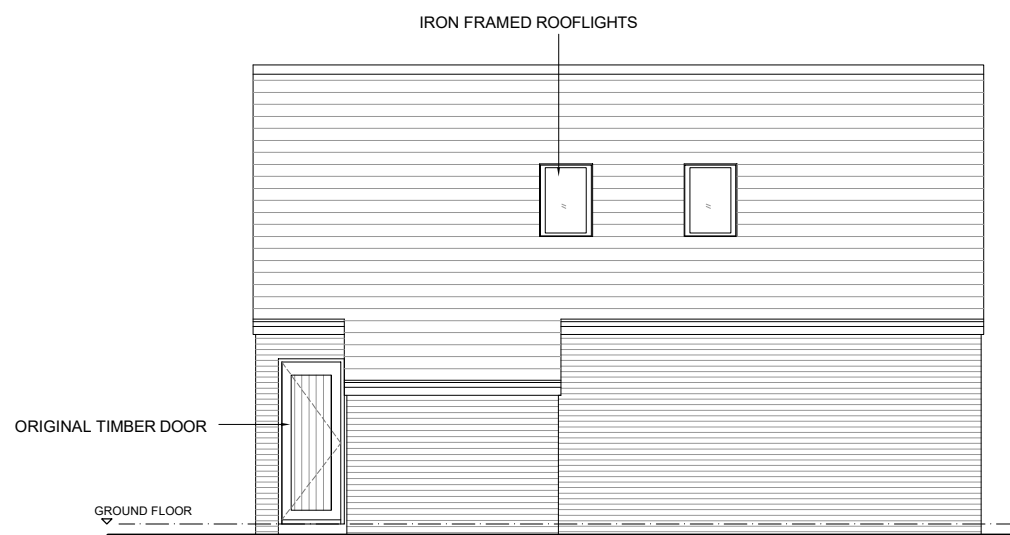
REAR ELEVATION
