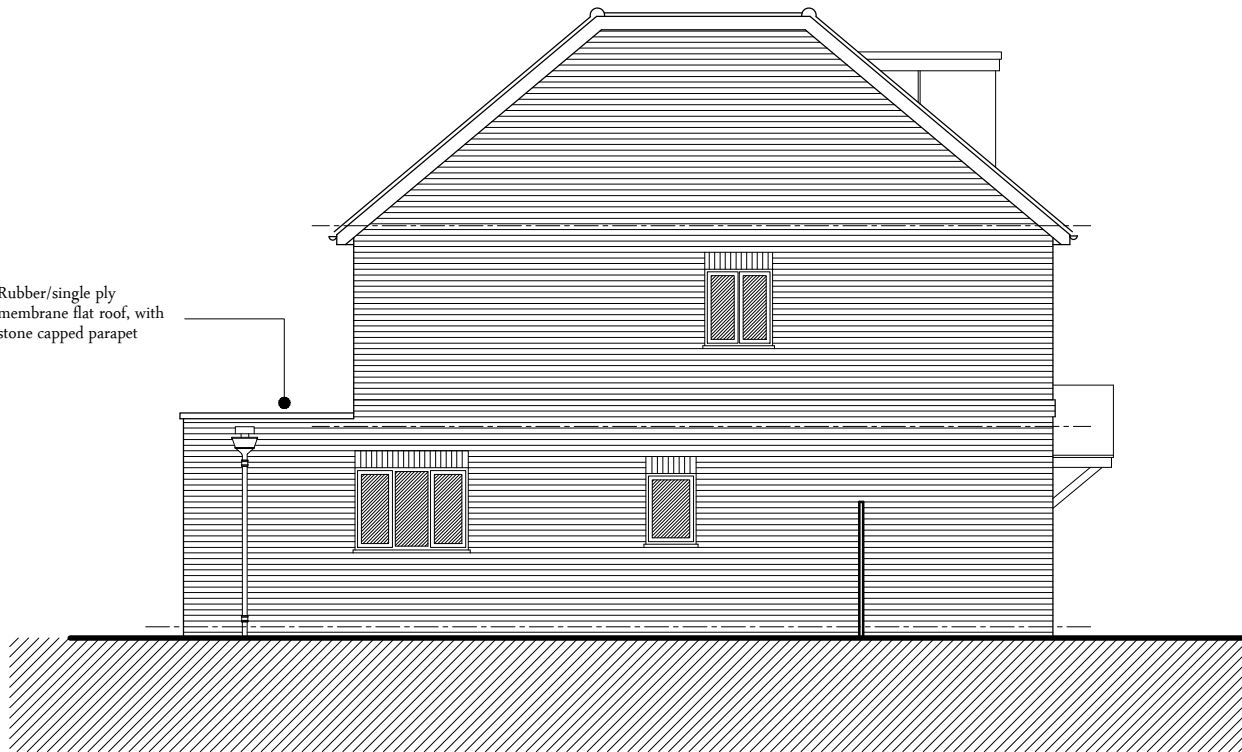
South Elevation
