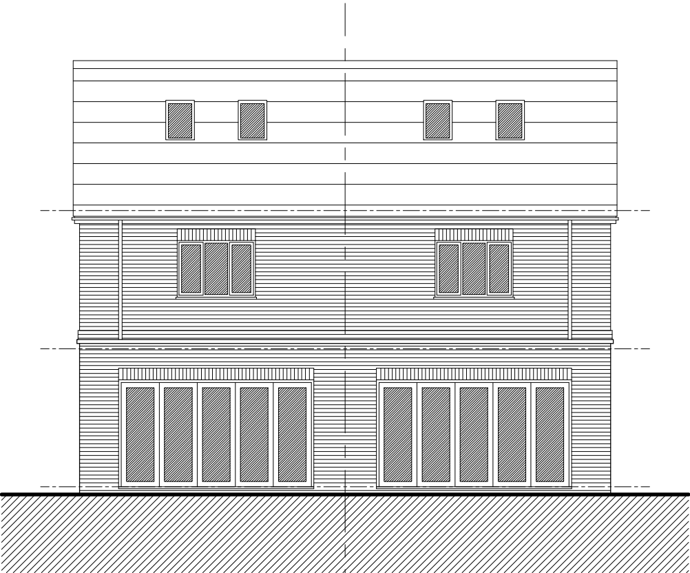
West Elevation
