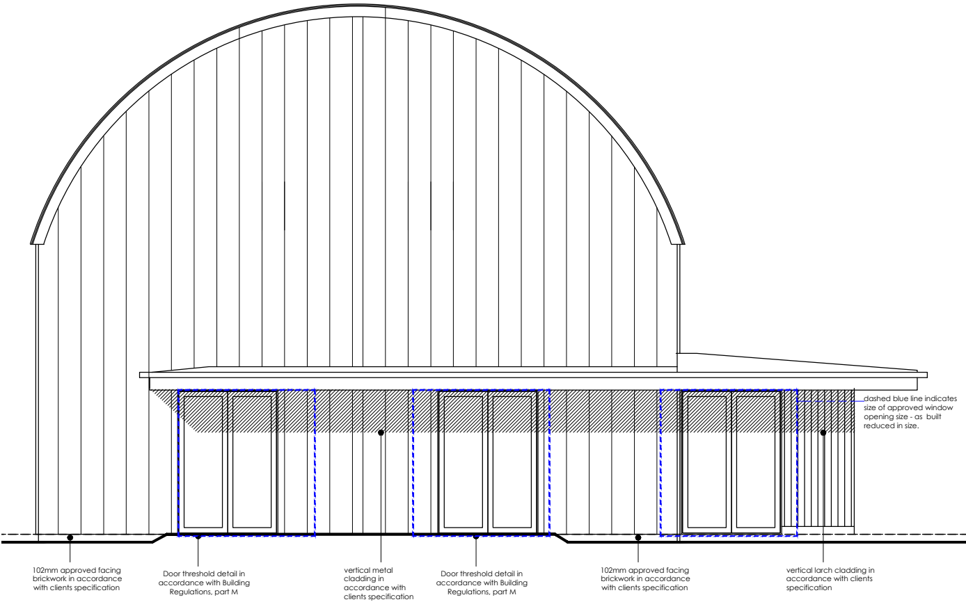
Existing elevation 03 1:100
