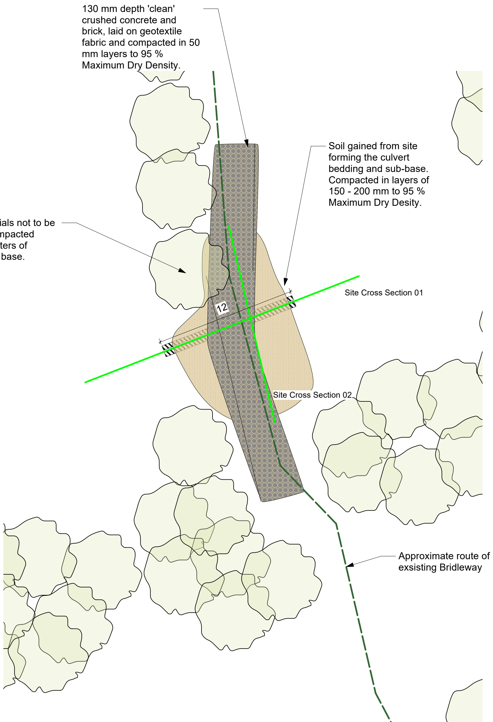
1 WILT18 Top/Plan Scale: 1:200
