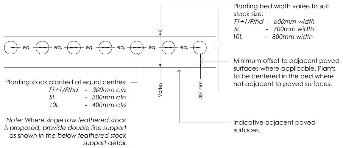
Detail 7 - Typical Single Row Hedgerow Layout (N.T.S.)
