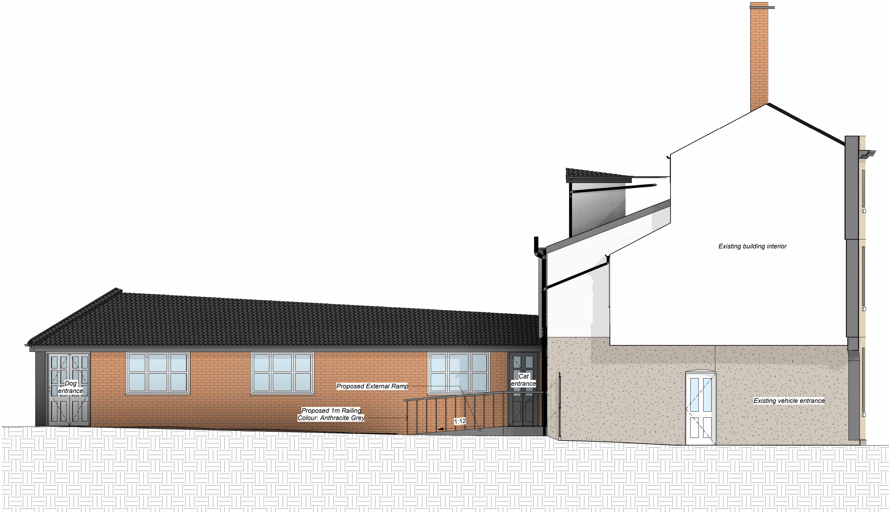
03 Side Elevation - Proposed 1 : 50
