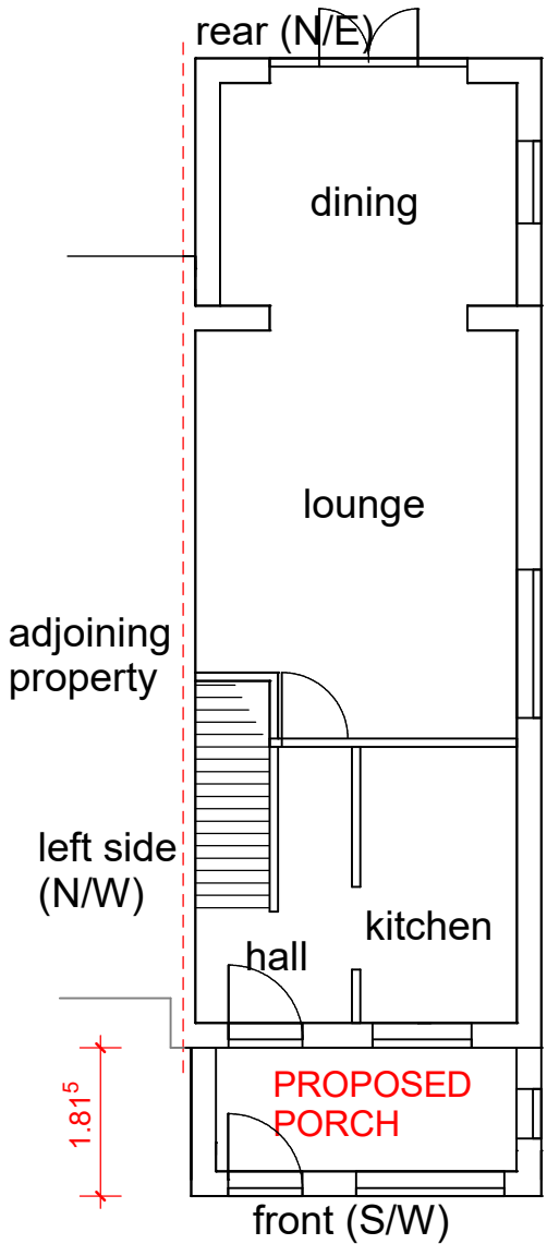
GROUND FLOOR LAYOUT
