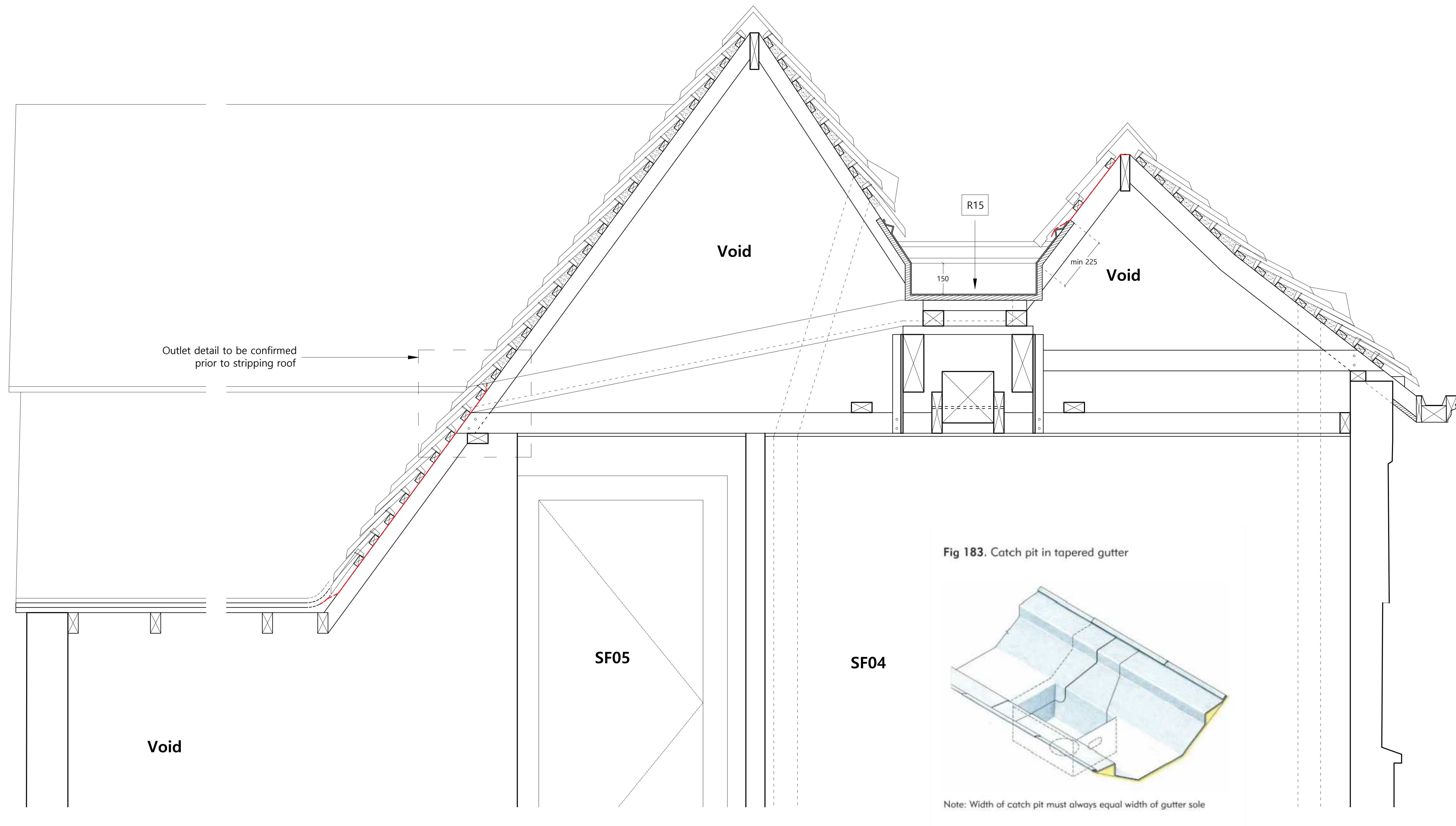
1.0 Section AA Showing Proposed Gutter
