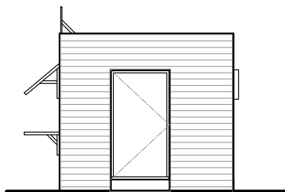
Proposed Side Elevation: 1:100 at A1 0m 1m 2m 5m 1:100
