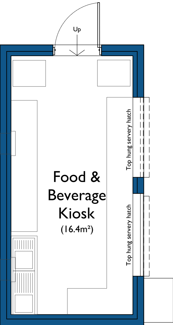
Proposed Floor Plan: Pre-fabricated Food & Beverage Kiosk 1:50 at A1 0m 0.5m 1m 2.5m 1:50
