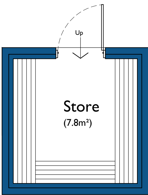
Proposed Floor Plan: Pre-fabricated Store 1:50 at A1 0m 0.5m 1m 2.5m 1:50
