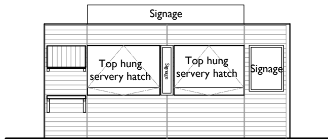
Proposed Front Elevation: 1:100 at A1 0m 1m 2m 5m 1:100 Materials Schedule: Walls: Horizontal overlap timber cladding Doors: Brown metal doors. Roof: Steel container roof (not visible).
