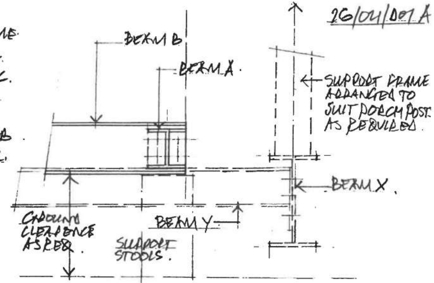
TYPICAL EDGE DETAIL
