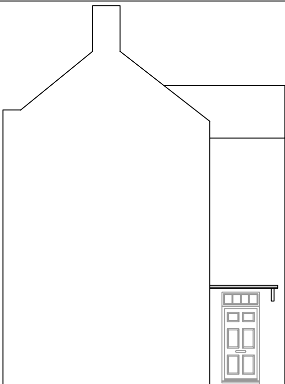
EXISTING RIGHT ELEVATION
