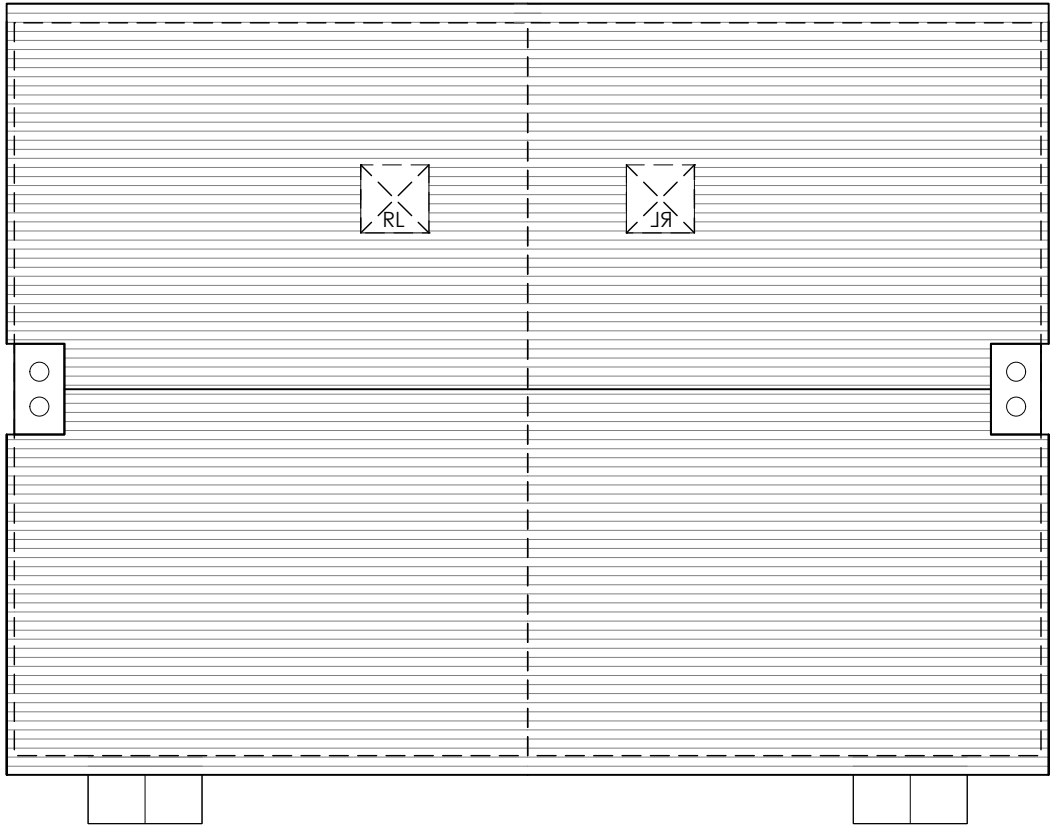
Roof Plan
