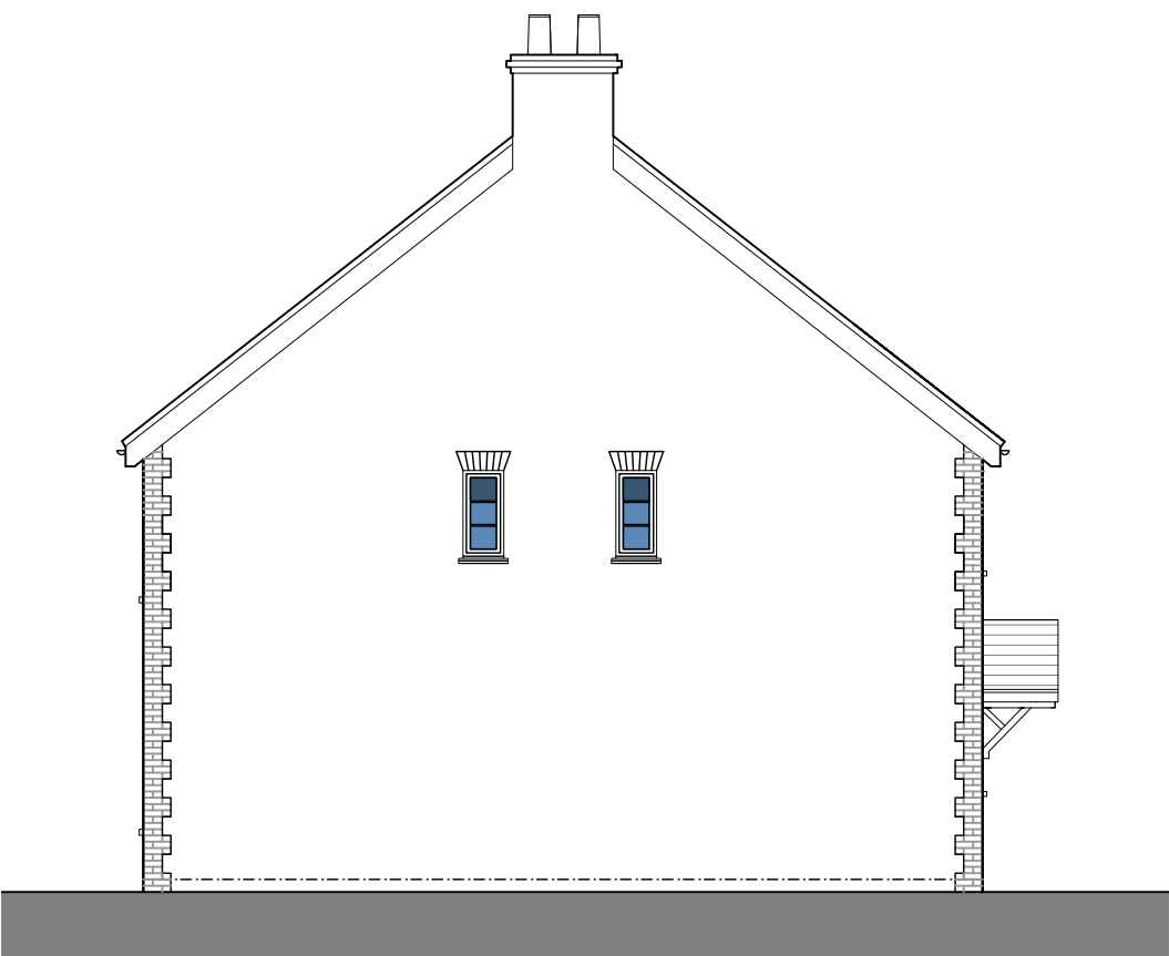
Side elevation
