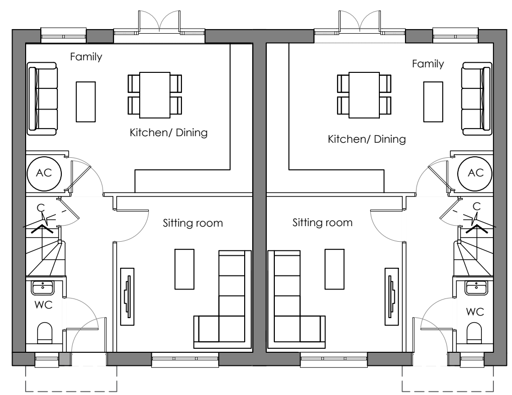
Ground Floor Plans
