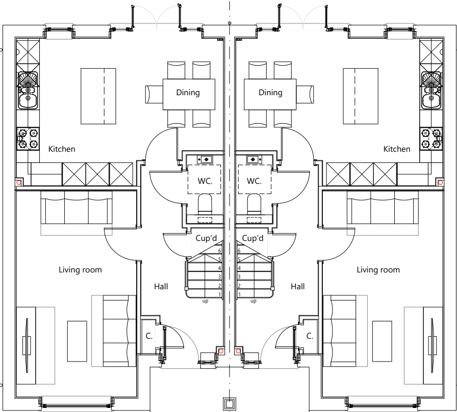
HT.SHER HT.SHER Ground Floor Plan
