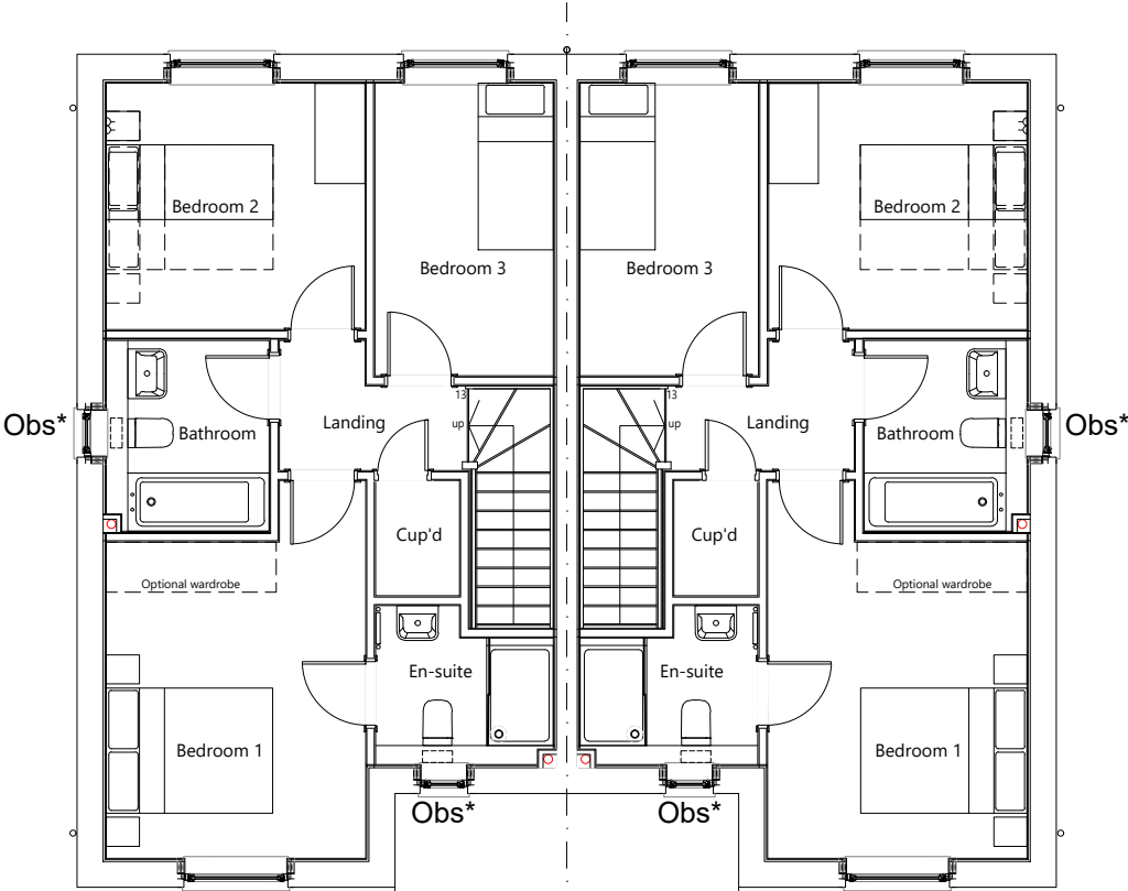
HT.SHER HT.SHER First Floor Plan Obs* - Obscure Window
