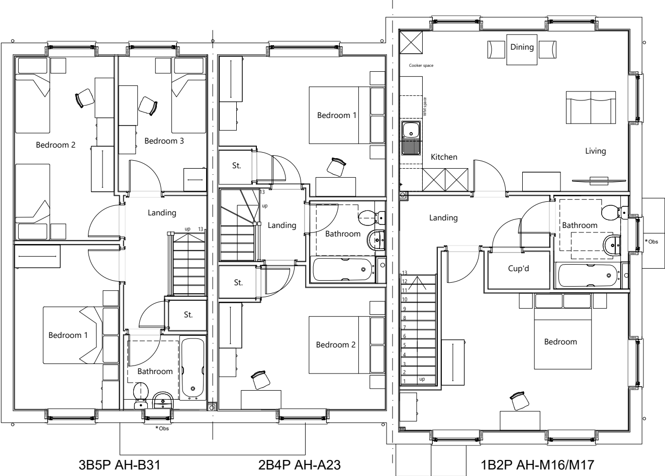
First Floor Plan Obs* - Obscure Window
