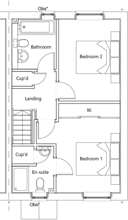
First Floor Plan Obs* - Obscure Window
