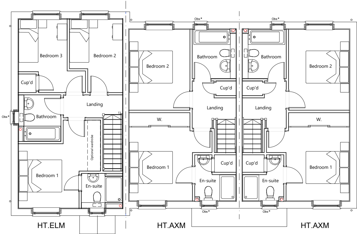
First Floor Plan Obs* - Obscure Window
