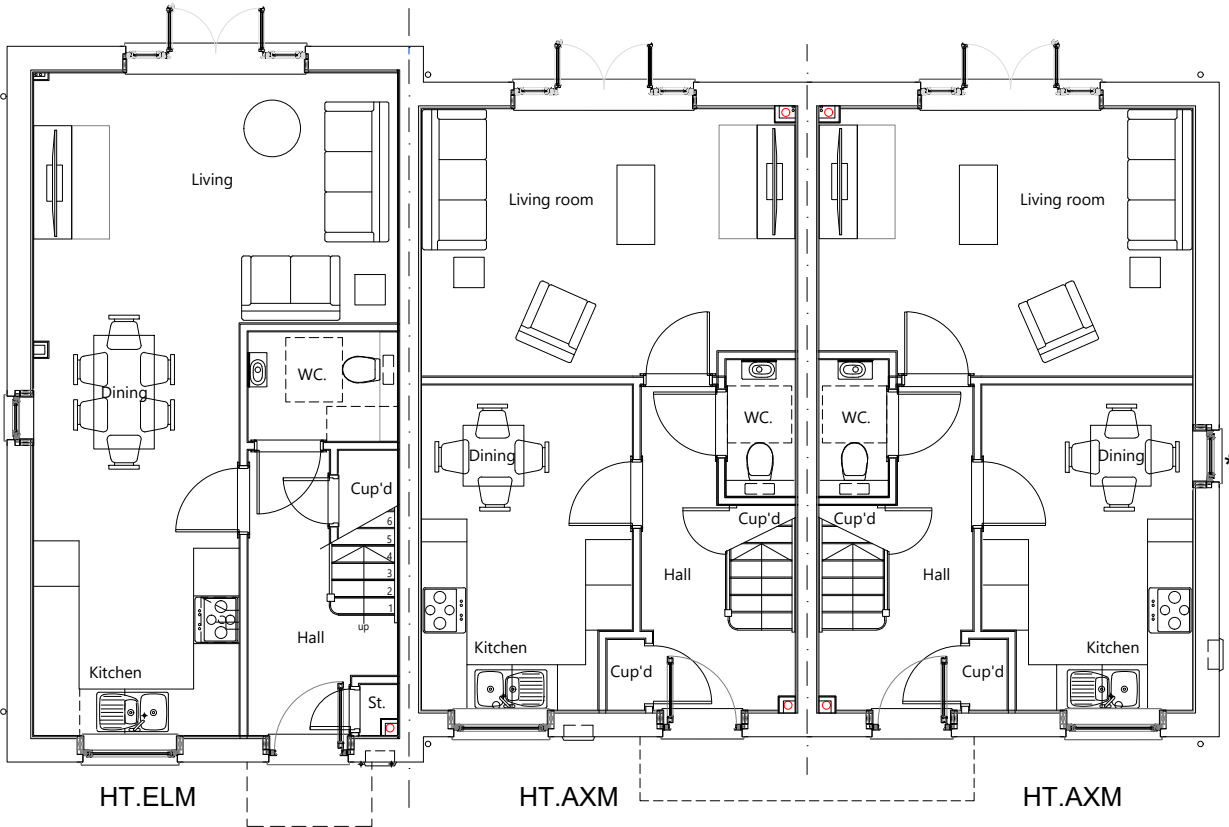
Ground Floor Plan *Side window for plot 41 only
