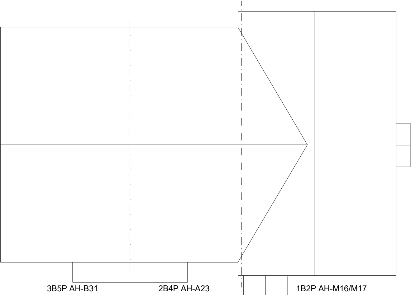
Roof Plan
