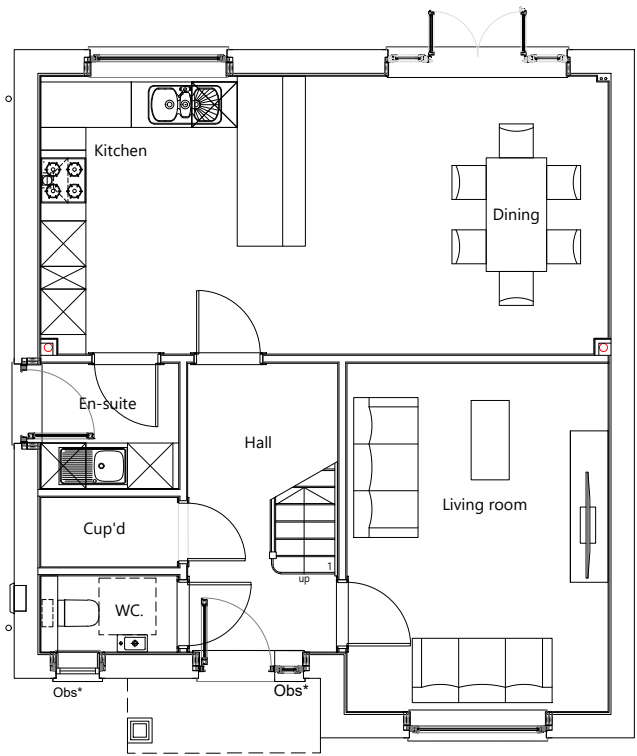
Ground Floor Plan Obs* - Obscure Window
