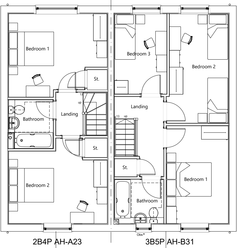
First Floor Plan Obs* - Obscure Window
