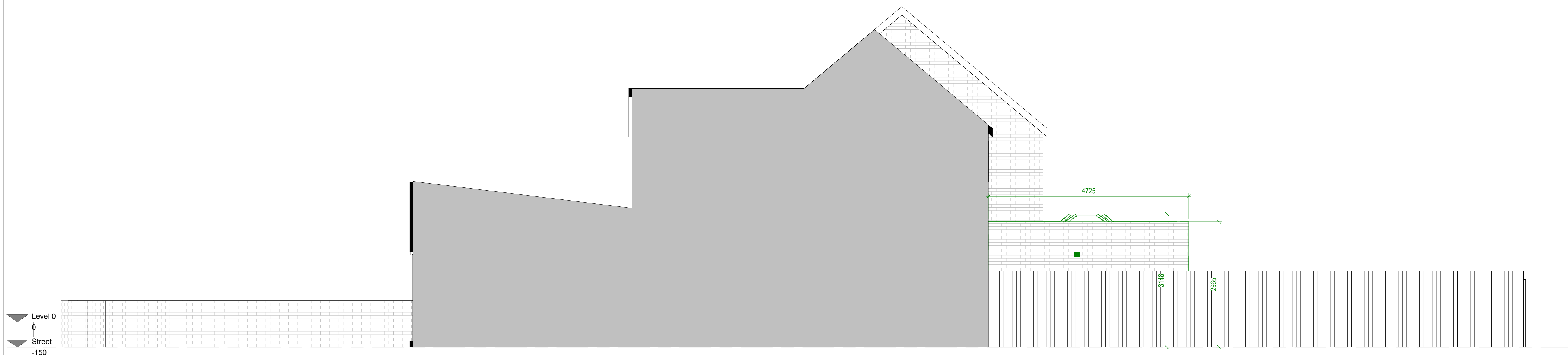
2 Proposed Side 2 Elevation 1 : 50
