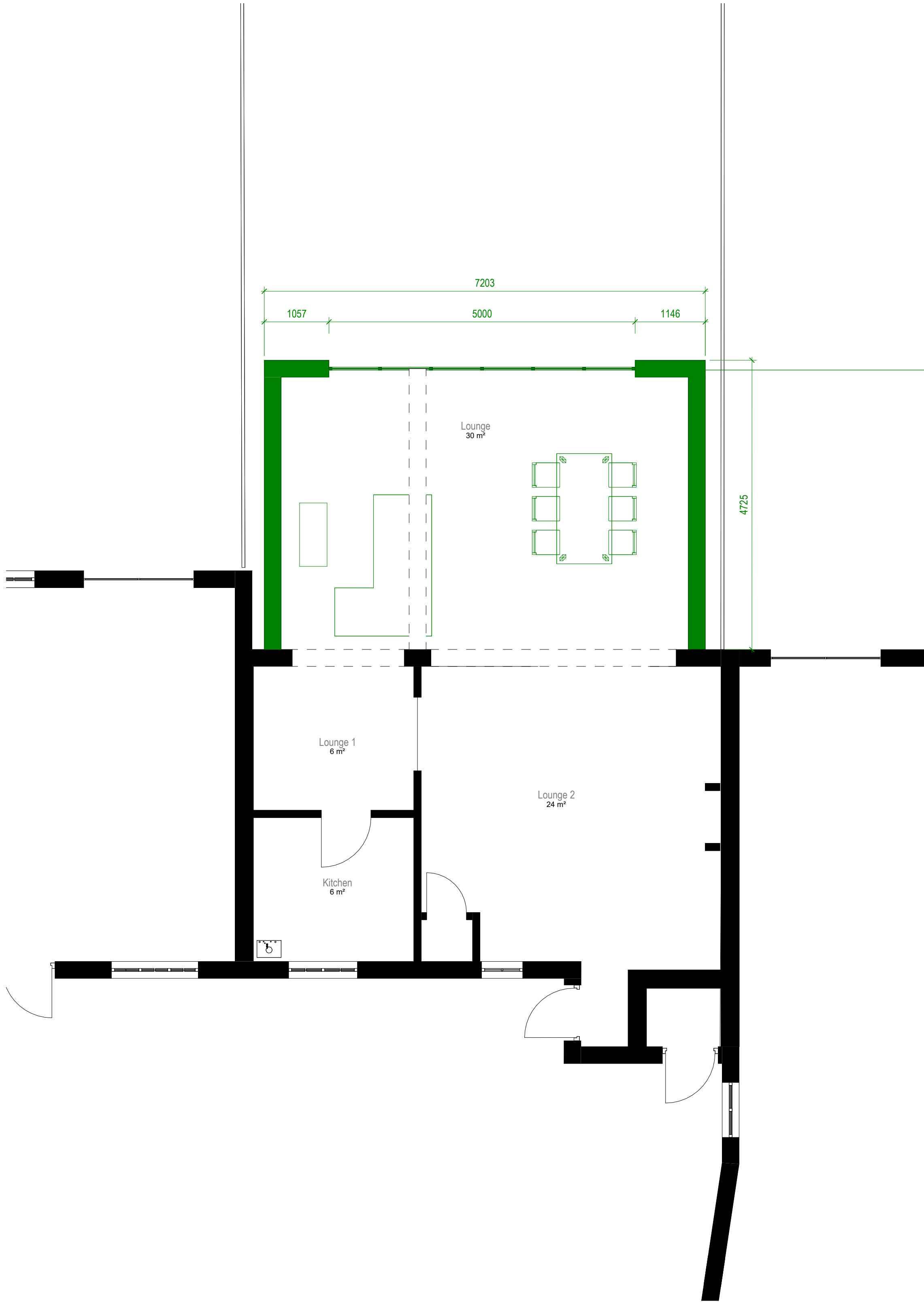
2 Level 0 Proposed 1 : 50
