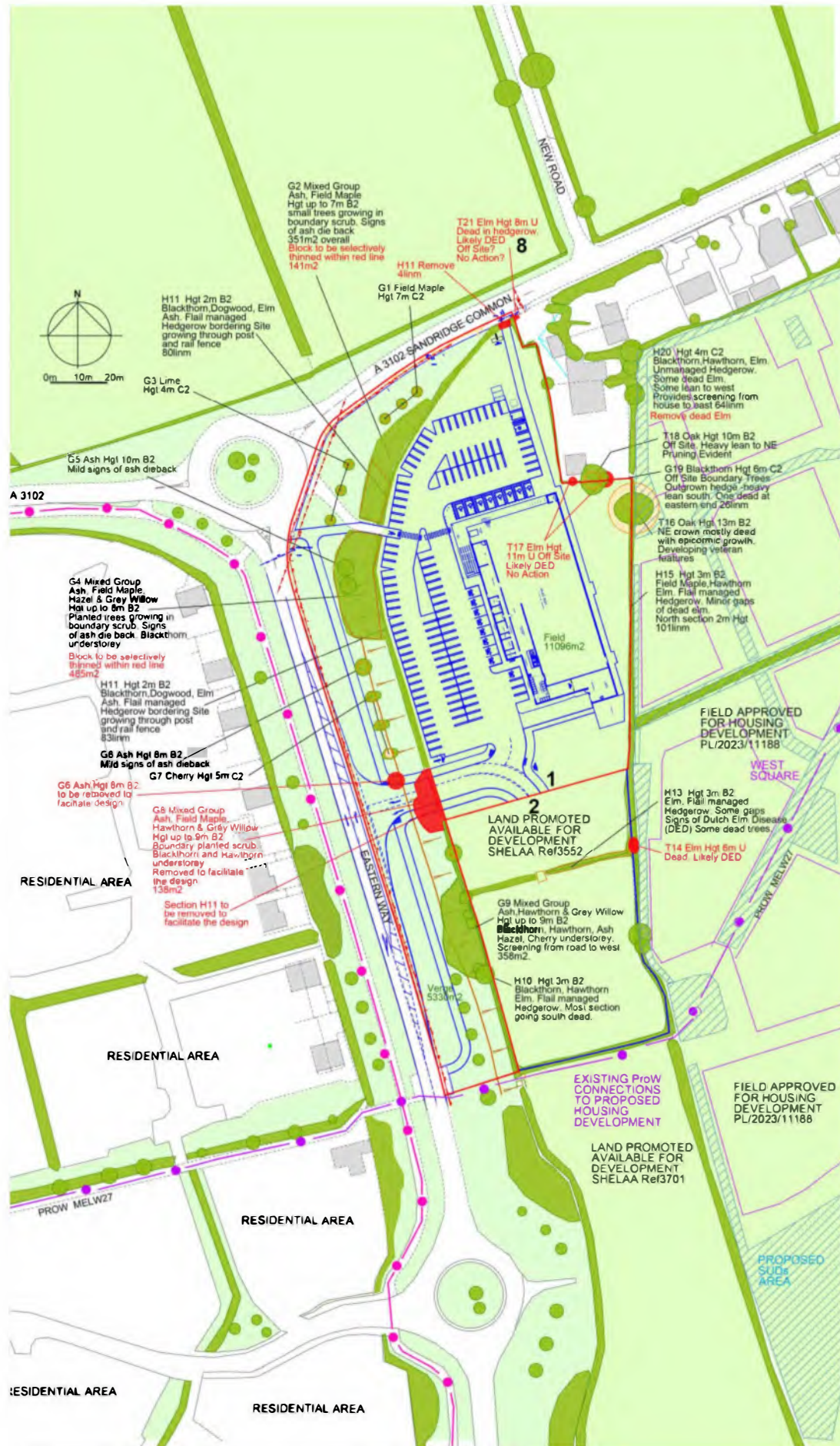
OVERALL SITE
