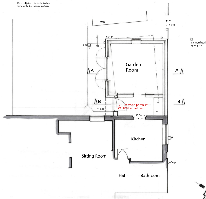
Ground Floor Plan 1-50 As Proposed
