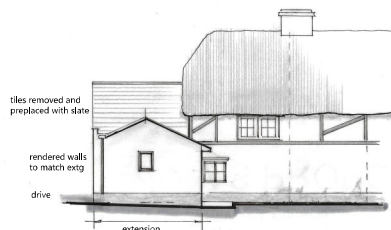
South West Elevation
