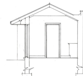
Section B-B 1-50
