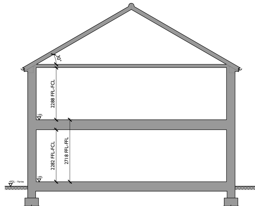
Section SFI - Plots 034/035 Truss Type A-30°
