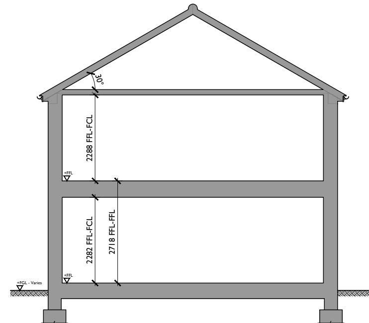
Section SFI - Plots 036/037 Truss Type A-30°
