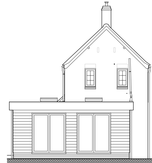
Proposed North East Elevation
