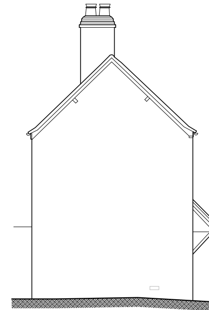
Existing South West Elevation
