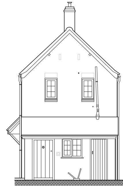
Existing North East Elevation
