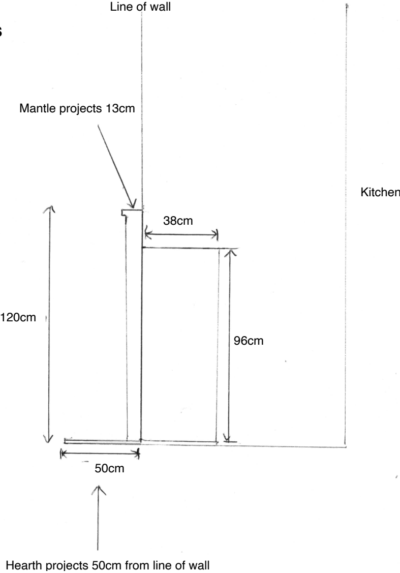
Side elevation
