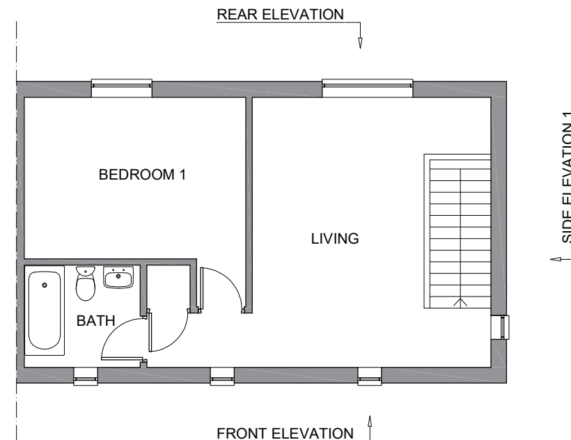
FIRST FLOOR PLAN AS EXISTING
