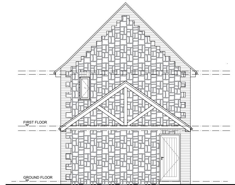
SIDE ELEVATION 1 AS EXISTING
