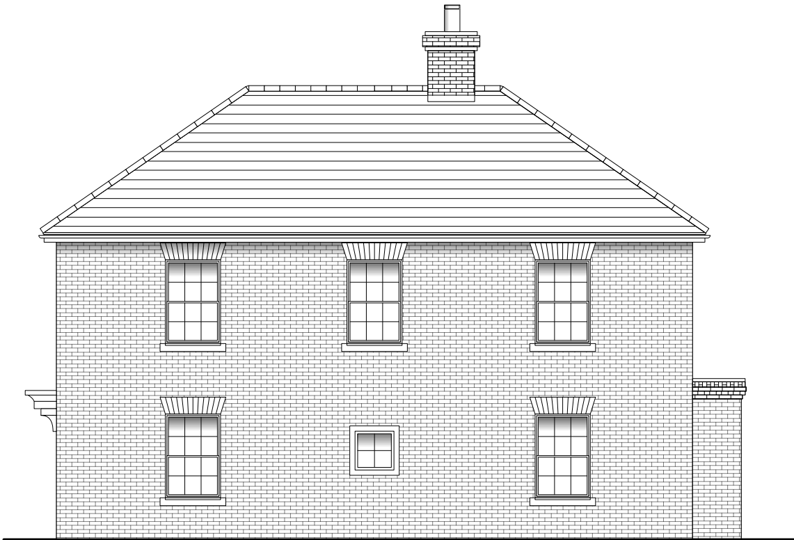
EXG. NORTH WEST ELEVATION 1:100
