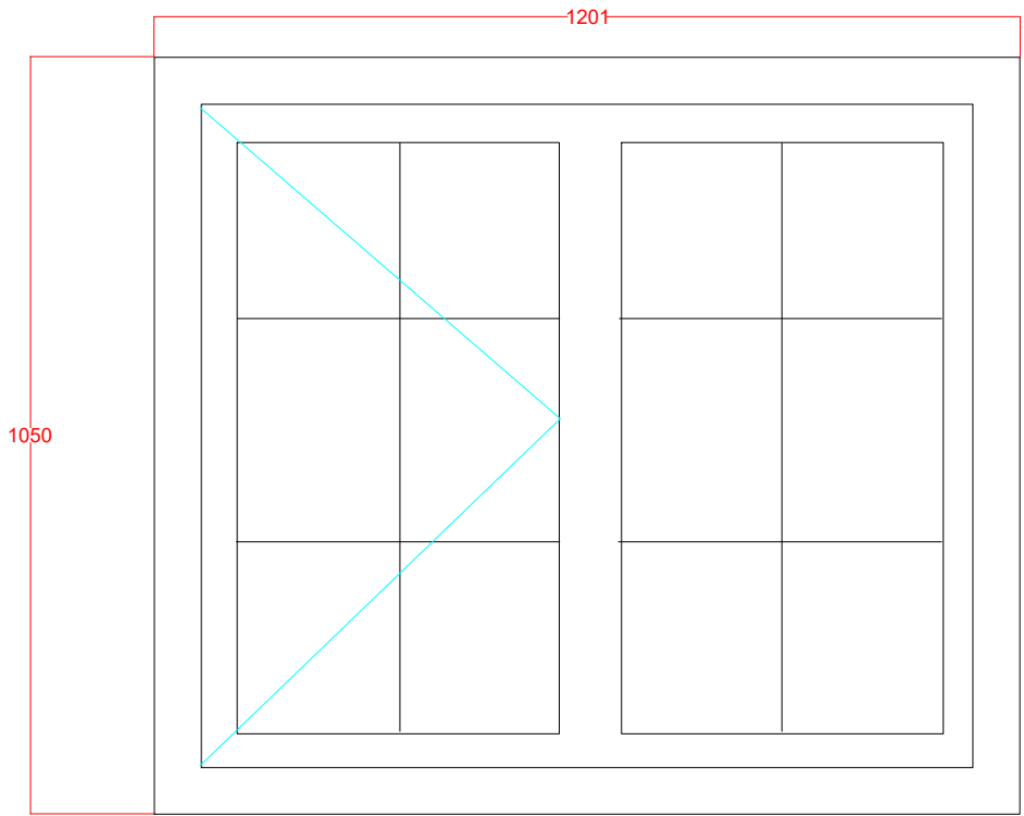
Window W3 First Floor North Elevation modern window to be replaced to match style of Window W1 and W2
