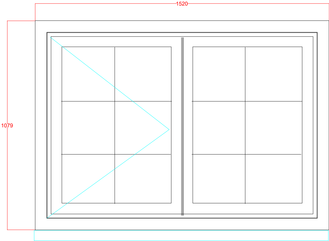
Window W2 North Elevation Ground Floor
