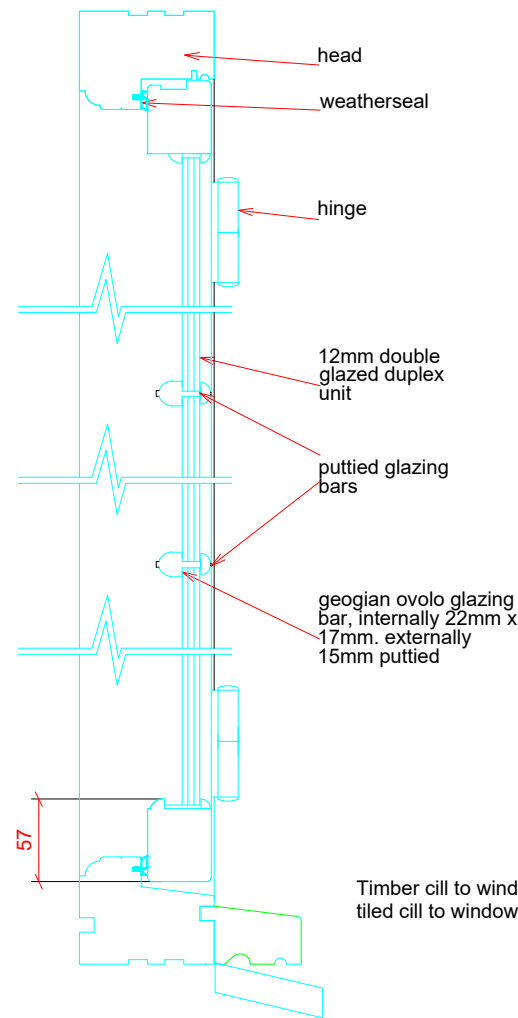
Existing tiled cill to windows W1 and W4 and replacement tiled window cill to window W2
