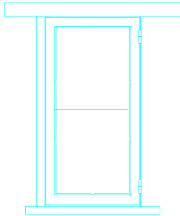
GROUND FLOOR WINDOW - WEST ELEVATION ref W5 740mm high by 410 wide slim line double glazed
