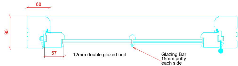
SIDE HUNG CASEMENT JAMB SECTION SCALE: 1:5 @ A3
