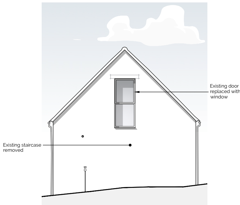
NORTH ELEVATION
