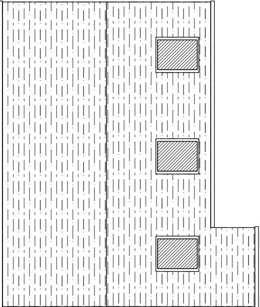
ROOF PLAN 1:100
