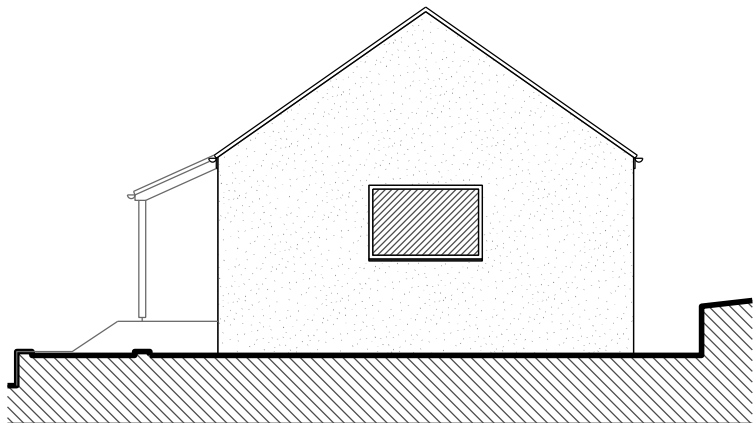
REAR ELEVATION 1:100
