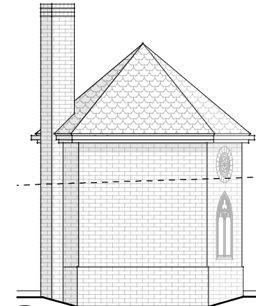
7 Proposed North Elevation Scale: 1:100
