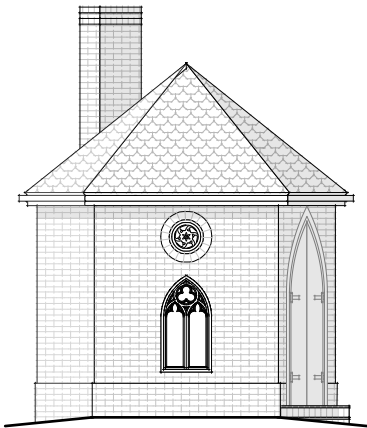
8 Proposed N-W Elevation Scale: 1:100
