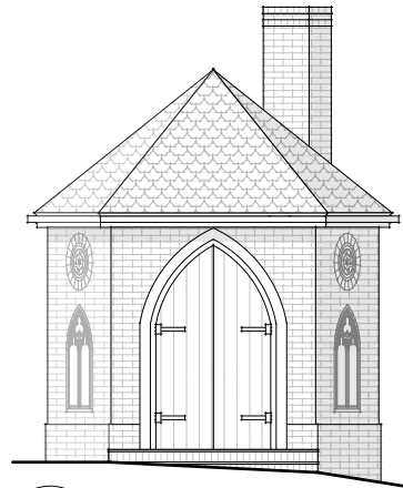
4 Proposed S-W Elevation Scale: 1:100
