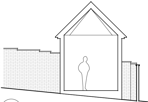
9 Proposed Section A-A Scale: 1:100
