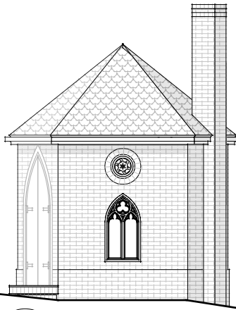
5 Proposed S-E Elevation Scale: 1:100
