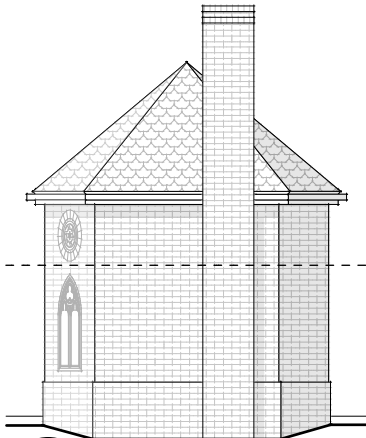
6 Proposed East Elevation Scale: 1:100
