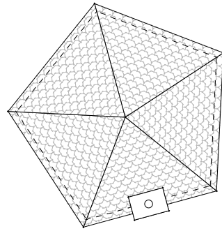
3 Proposed Roof Plan Scale: 1:100
