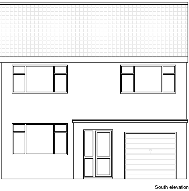
South elevation
