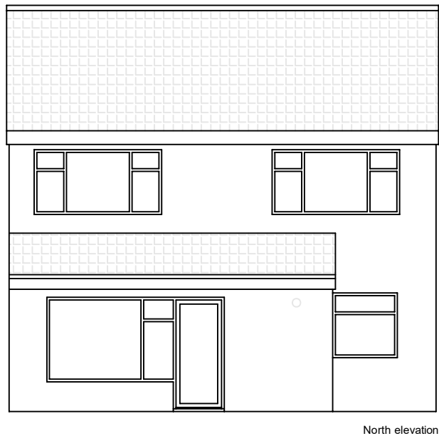
North elevation
