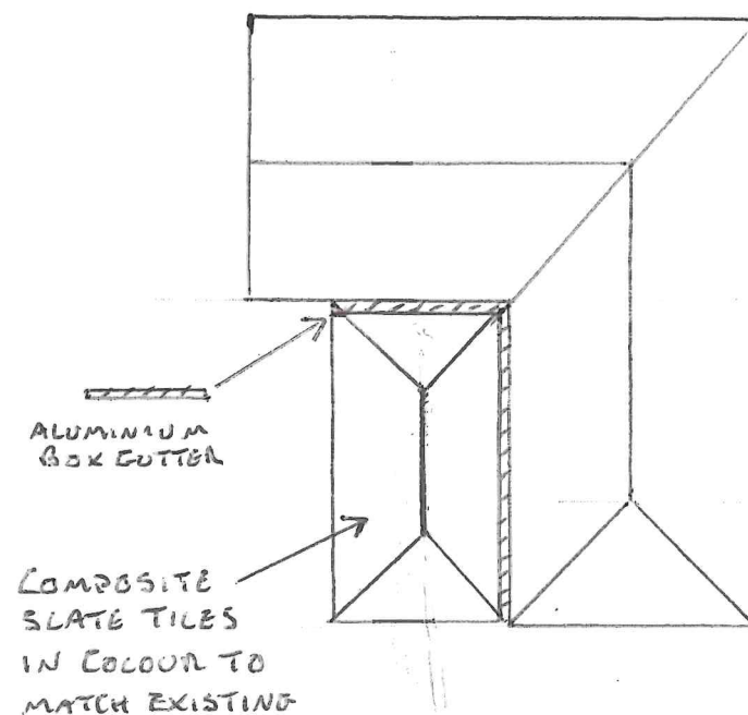
PROPOSED ROOF PLAN 1-200
