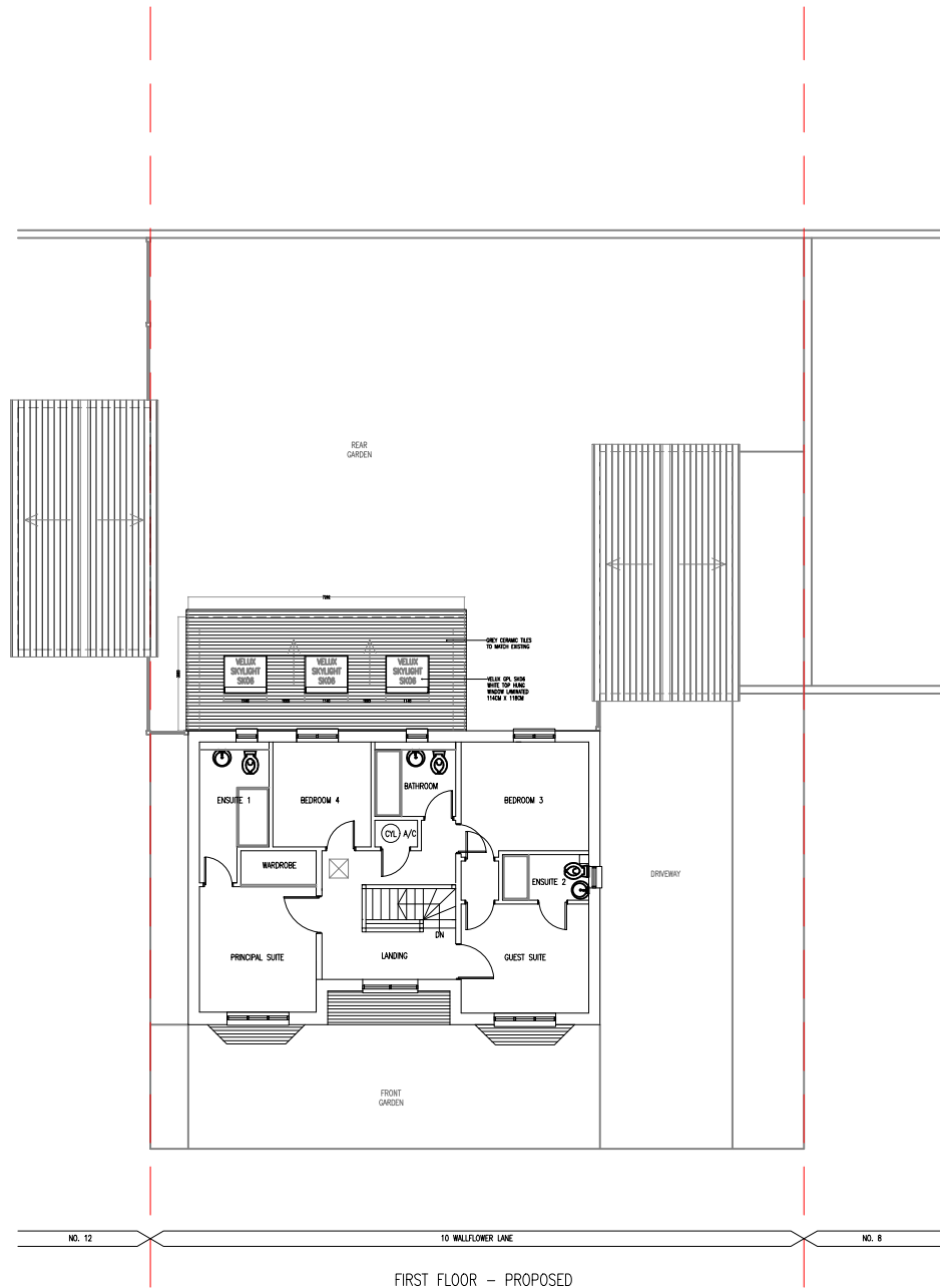
FIRST FLOOR – PROPOSED
