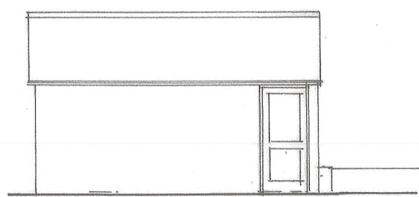
East Elevation
