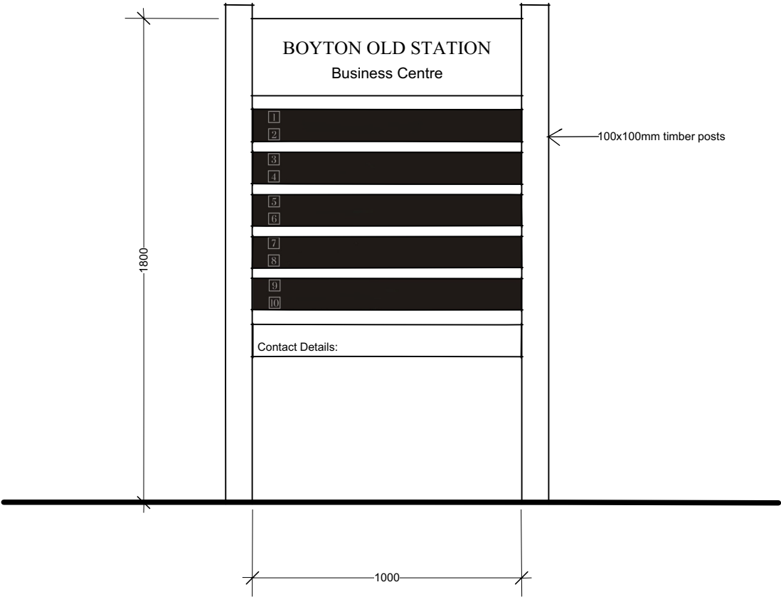
Front (Road Facing) Elevation
