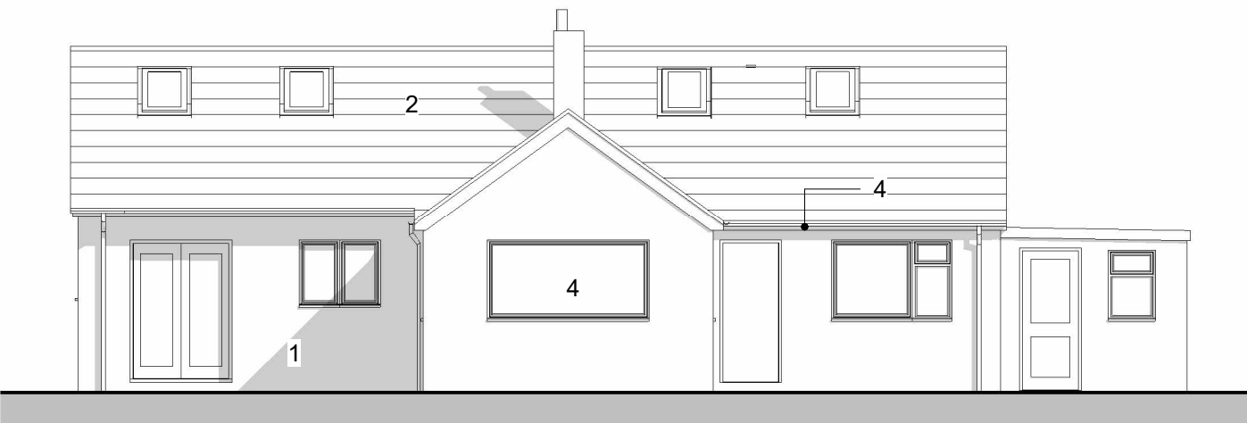
4 | Existing South West Elevation (Rear) 1 : 100
