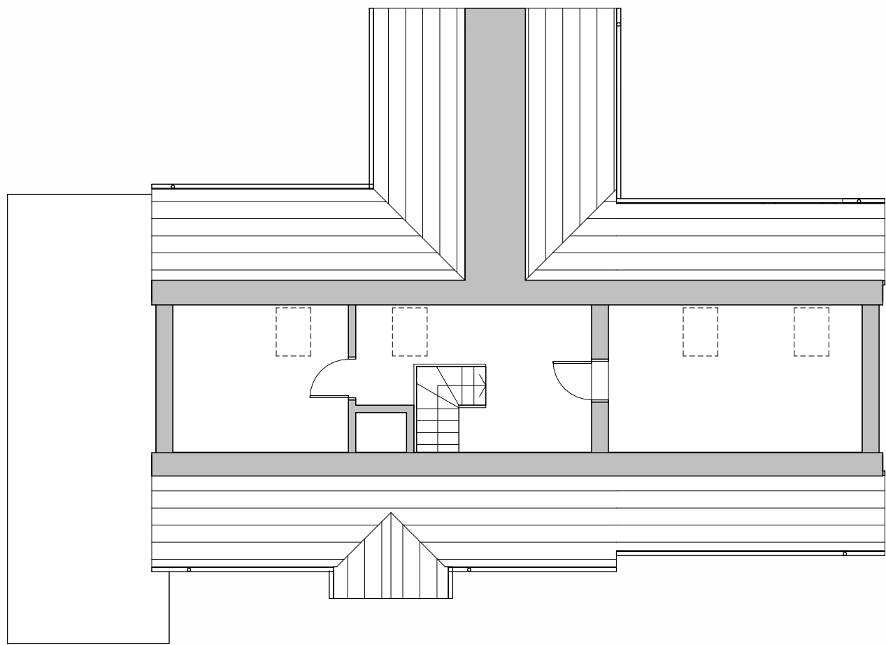
2 | Existing First Floor 1 : 100
