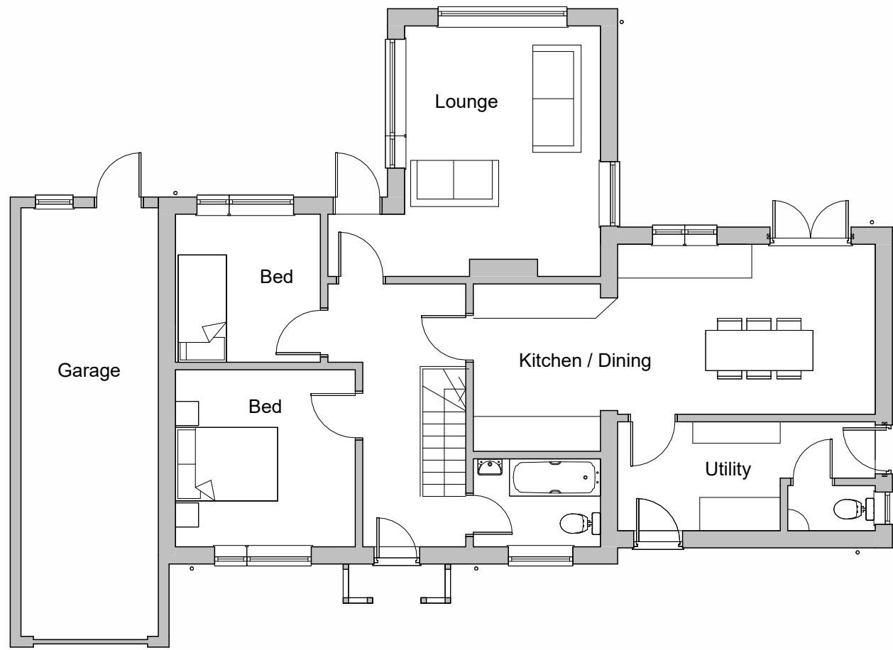
1 | Existing Ground Floor 1 : 100
