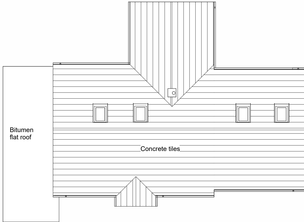
3 | Existing Roof Plan 1 : 100
