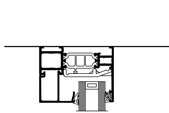
1:2 Head Detail
