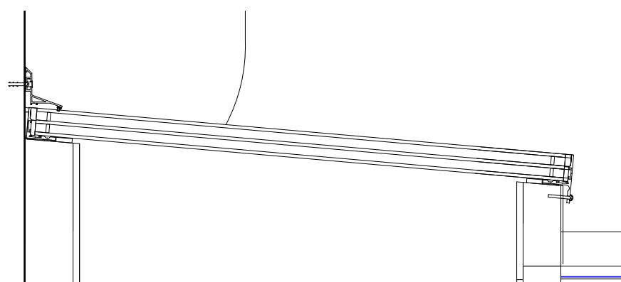
1:20 Section RL02 - Flat roof abutment glazed rooflight Powder coated aluminium
