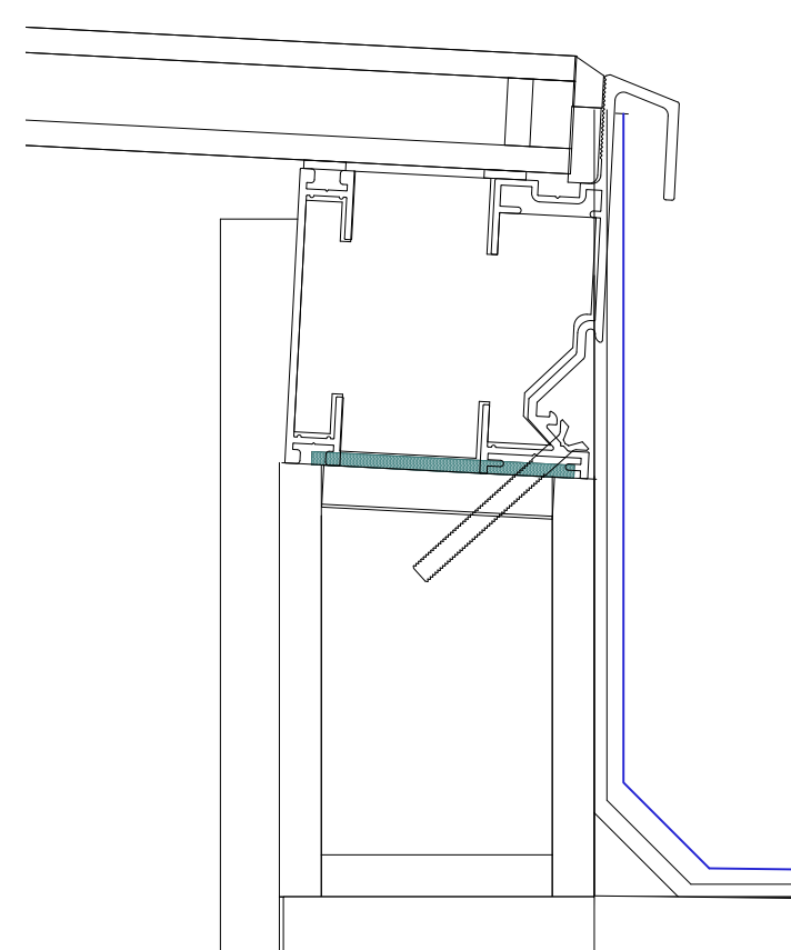
1:2 Frame Detail
