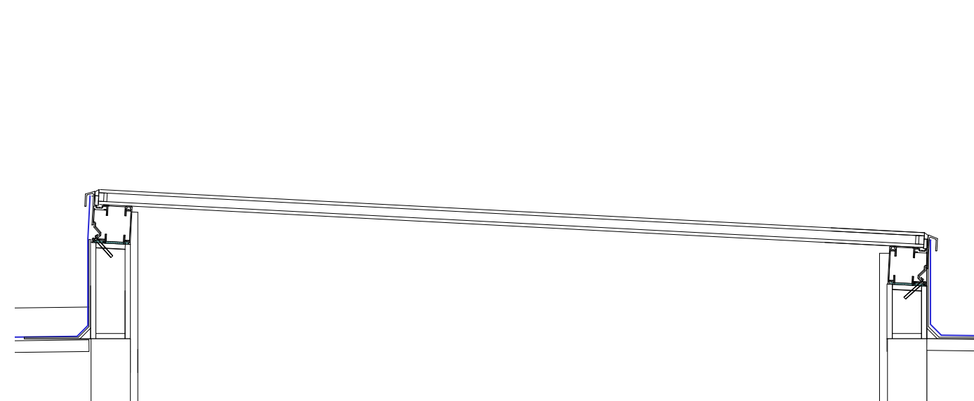
1:20 Section RL01 - Flat roof glazing rooflight Powder coated aluminium
