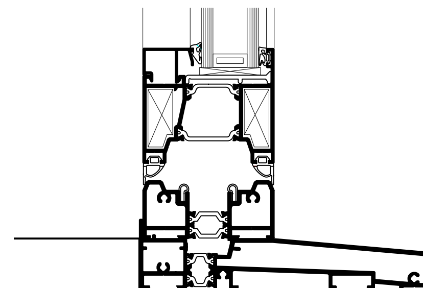
1:2 Cill Detail
