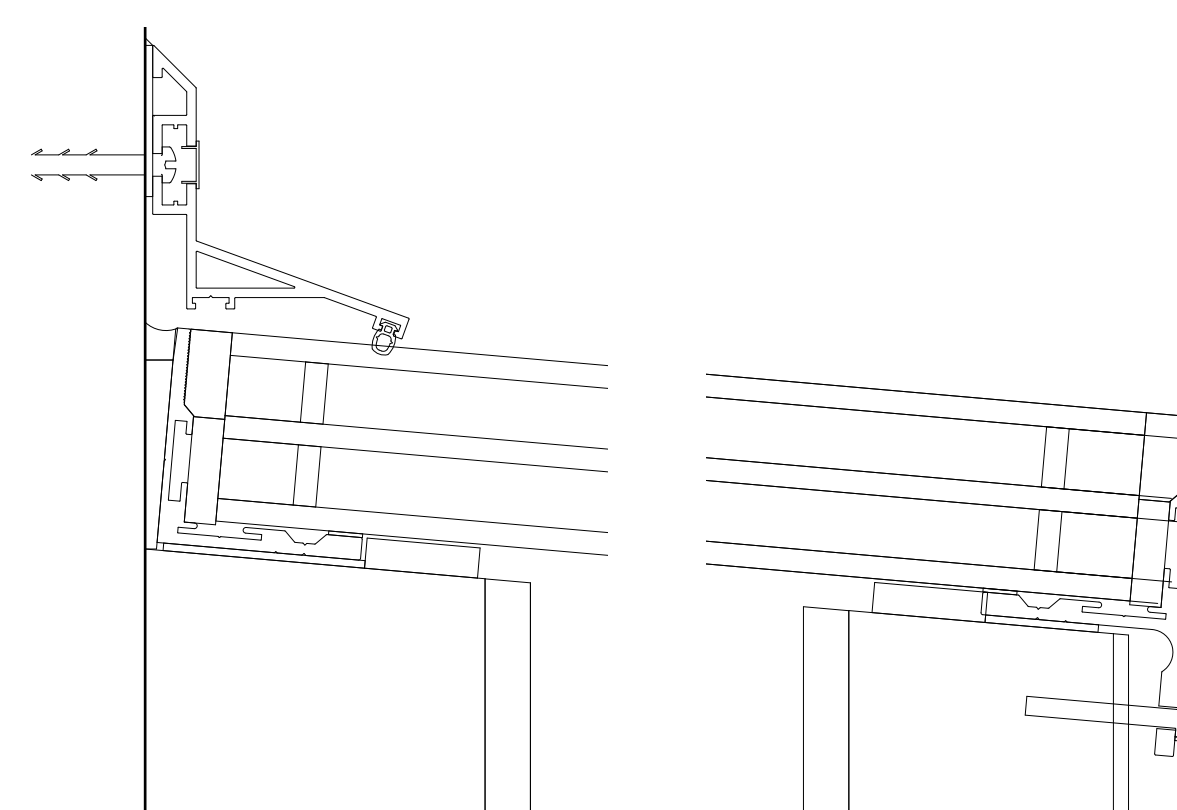
1:2 Frame Detail
