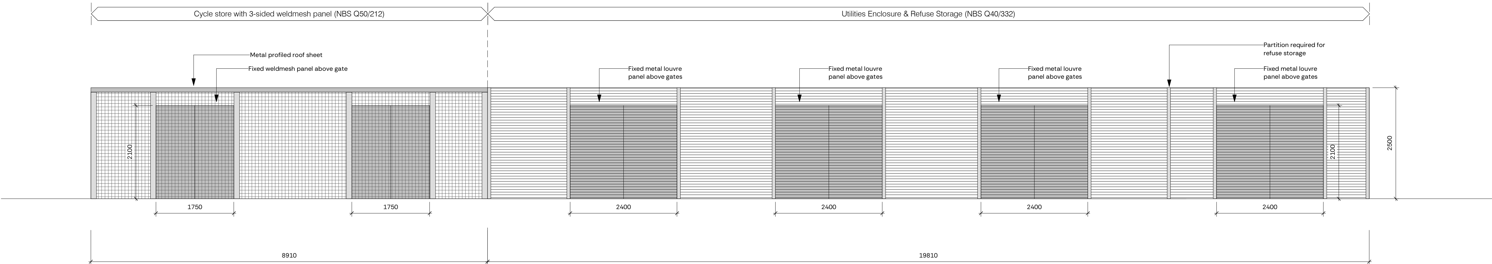
Cycle Store, Utilities Enclosure and Refuse Storage Front Elevation 1: 50
