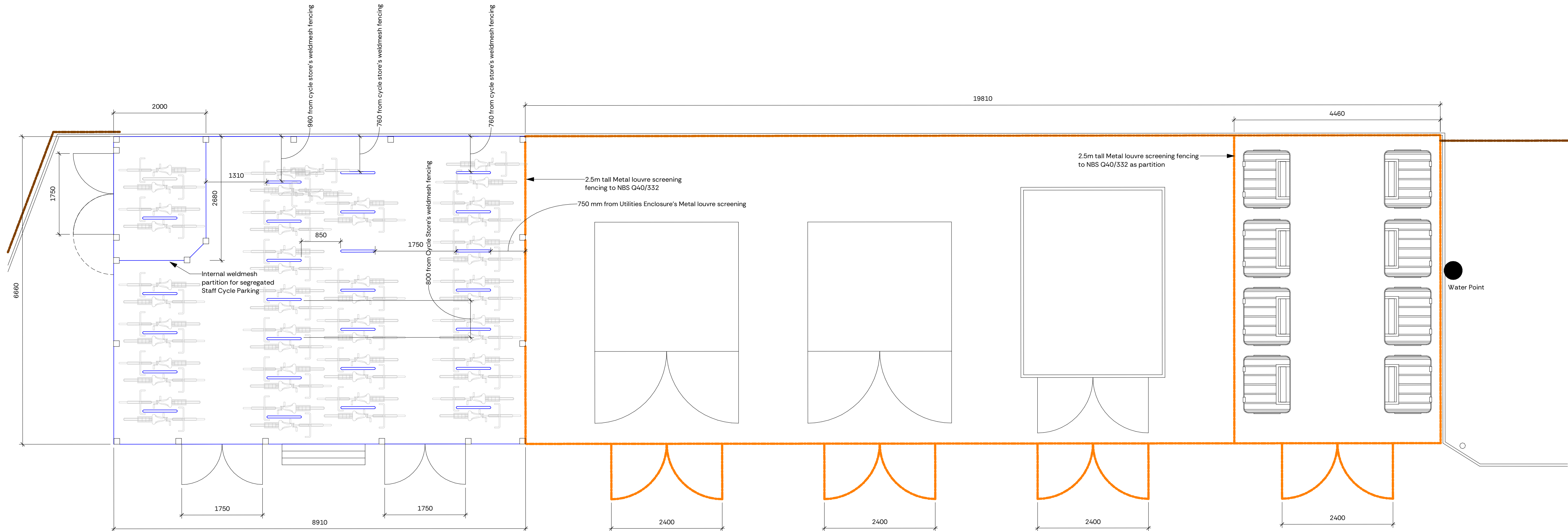
Cycle Store , Utilities Enclosure and Refuse Storage Plan 1: 50
