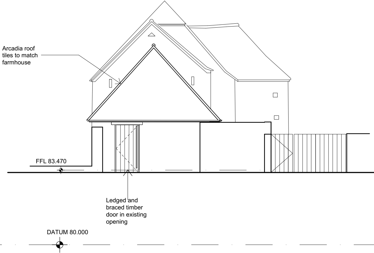
WEST ELEVATION
