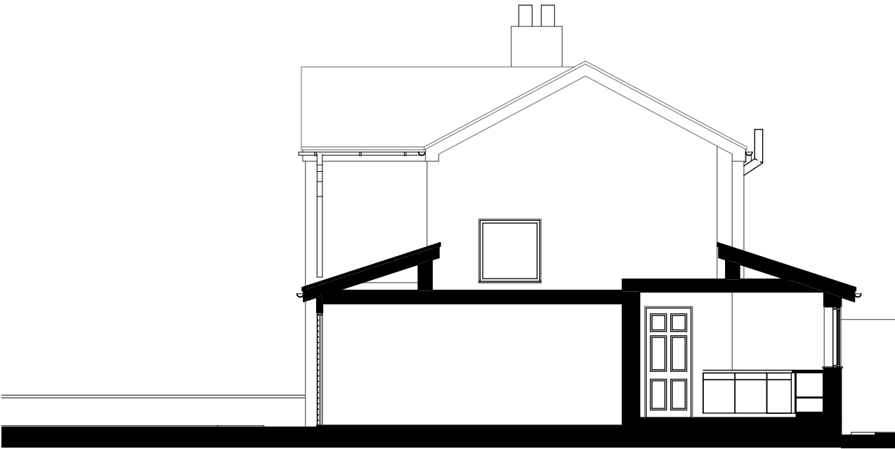
S-01 Building Section 1:100
